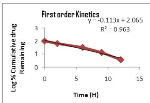
FIGURE: IV First order release kinetics
