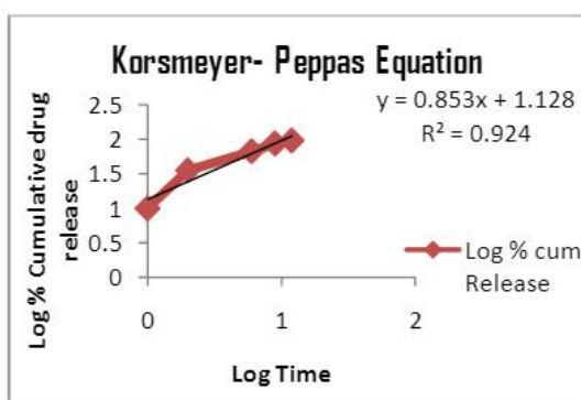
FIGURE: VI Korsmeyer- Peppas release kinetics
