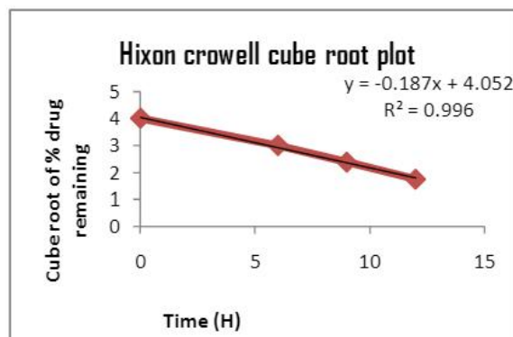
FIGURE: VII Hixon crowell release kinetics
