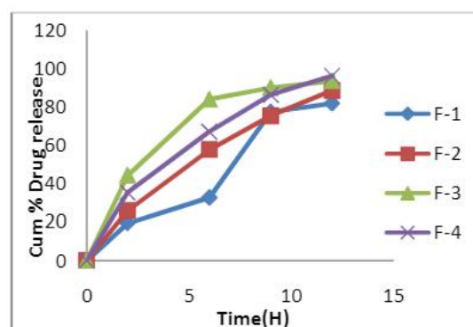
FIGURE: II Release profile for Doxofylline as sustained release
