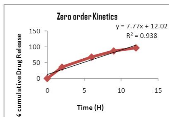
FIGURE: III Zero order release kinetics
