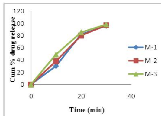
FIGURE: I Release profile for Montelukast sodium as immediate release
