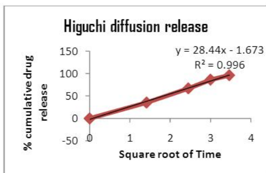
FIGURE: V Higuchi release kinetics
