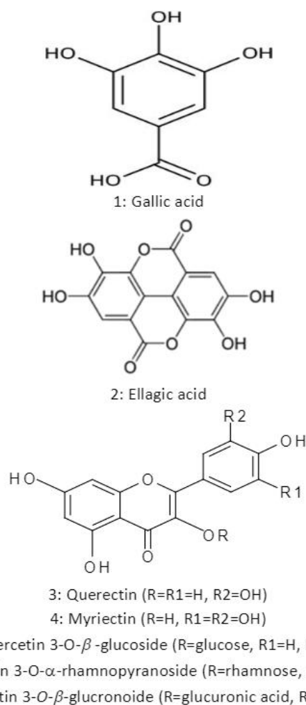
Figure 1. Chemical structures of the compounds isolated from D. kaki peels methanol extract
