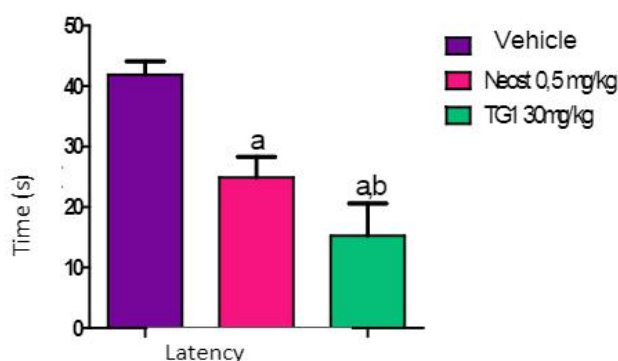
Figure 4 - Latency (s) on test day (day 4) to reach the location on training days the platform was located. Data are expressed as mean \pm standard error. a p \leq 0,05 compared to the vehicle group and b p \leq 0,05 compared to the control group.
